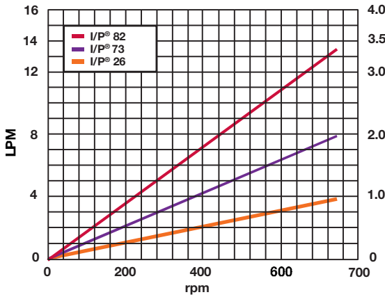
Flow Curves I/P® Easy-Load® Pump
