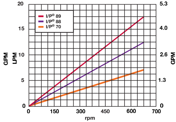
Flow Curves I/P® High-Performance Pump
